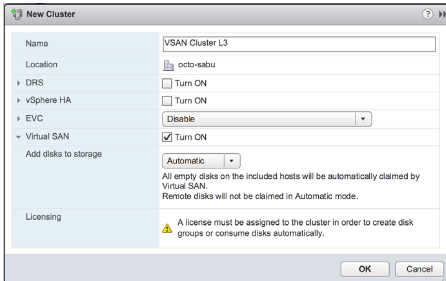
Figure 12: Enable Virtual SAN
